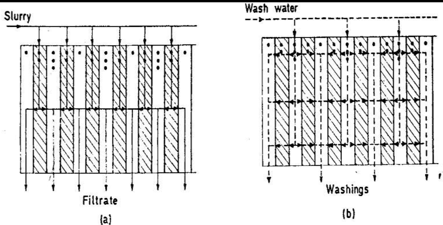
Fig. 20.6 Washing plate and frame filter press: principles of operation (a) filtering (b) washing
